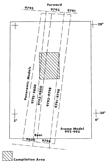
FIG. 2. Photo index showing panoramic and frame model coverage over compilation area.
