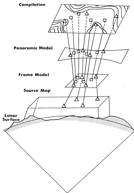
FIG. 6. Development of compilation control.
