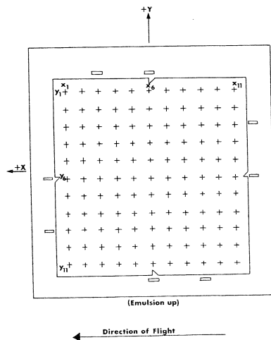
FIG. 7. Calibrated grid used on frame photographs.
